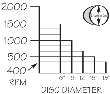
FACEPLATE TURNING
